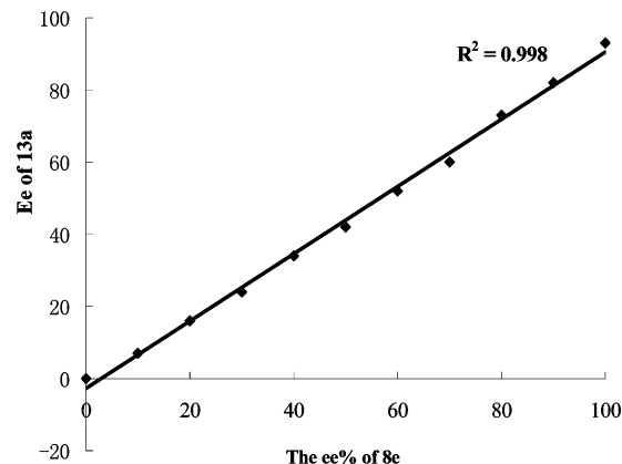
FIGURE 2. Linear relationship between enantiomeric excesses of product 13a and catalyst 8e in the direct aldol reaction of benzoylformic acid ( 2a ) with acetone in toluene.
