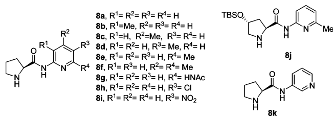
FIGURE 1. Organocatalysts used in this study.
